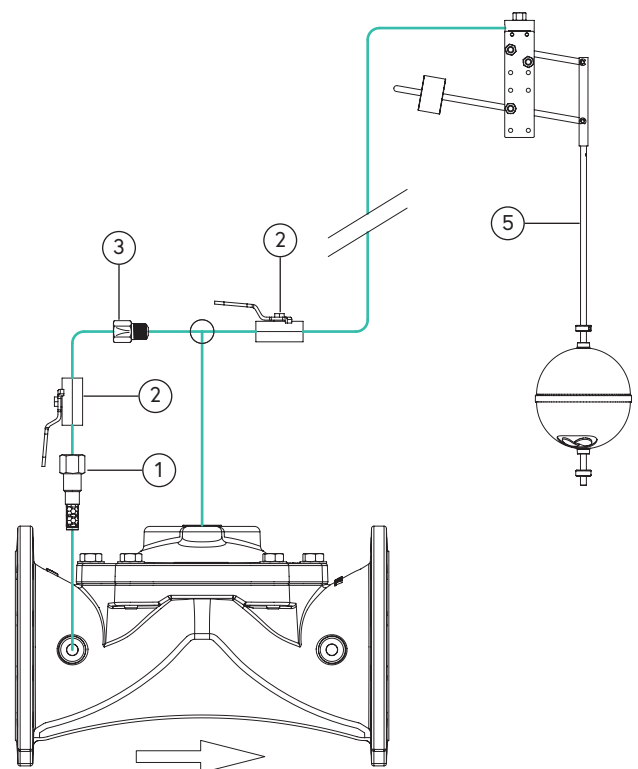
Level control Valve - Vertical Float
