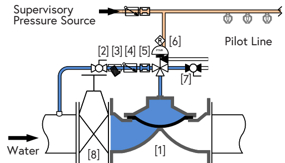
Pneumatically Actuated
