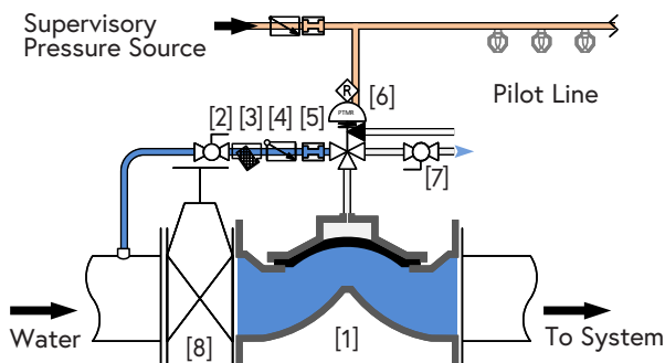
Manually Actuated
