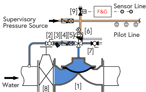
Standby Position
