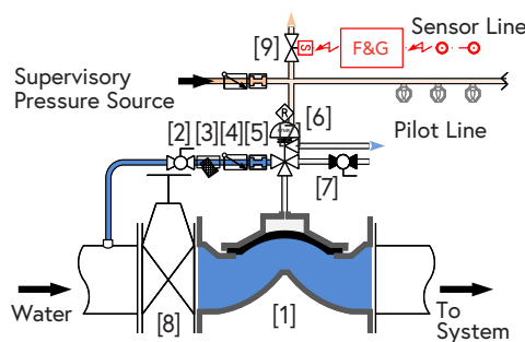
Electrically Actuated
