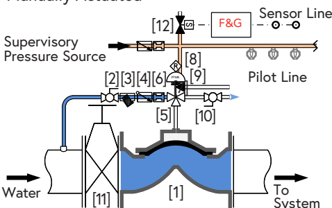
Manually Actuated
