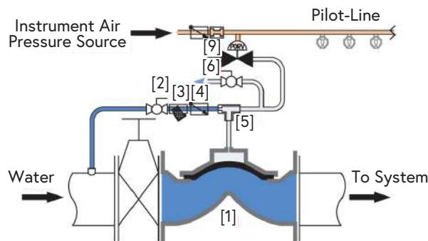
Manually Actuated
