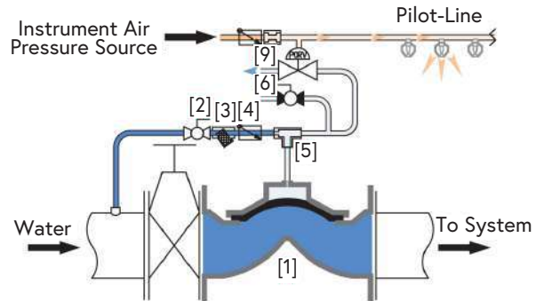
Pneumatically Actuated
